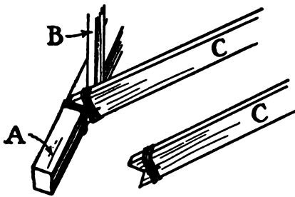
FIG. 27. — Detail of Diagonal Braces.
